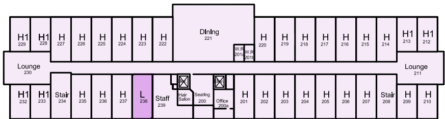
2nd Flr.Keyplan
