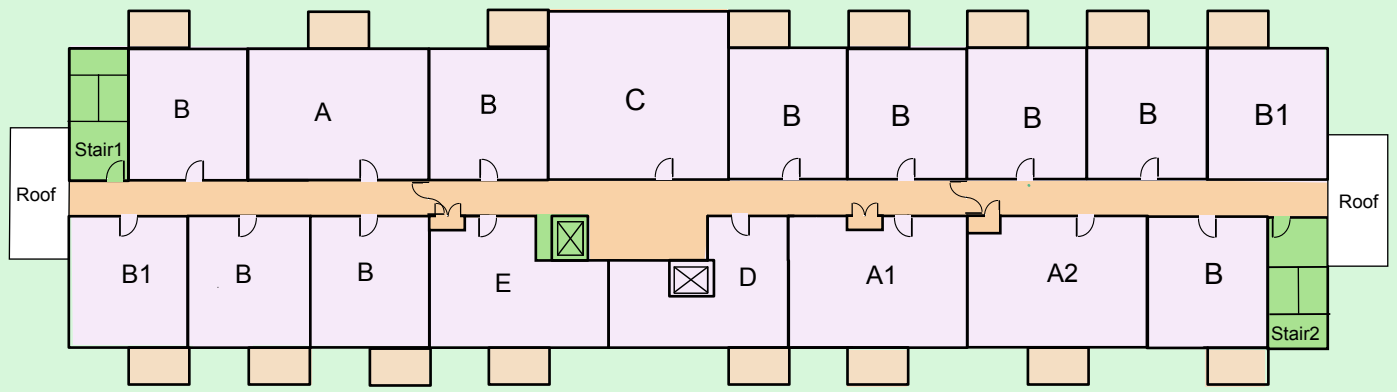
Third Floor 16 Units 18,361 SF
